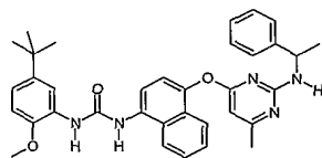
1-(5-tert-Butyl-2-methoxy-phenyl)-3-{4-[6-methyl-2-(1-phenyl-ethylamino)-pyrimidin-4-yloxy]-naphthalen-1-yl}-urea;
